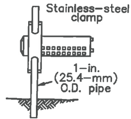
Strainer support clamp #230
