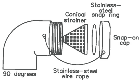
Dry hydrant head #227 [Specify 90 degrees, 45 degrees, or straight and 4½-in.(114-mm), 5-in.(127-mm), or 6-in.(152-mm) NH male thread]
